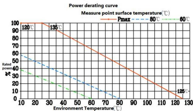
500W Attenuator
