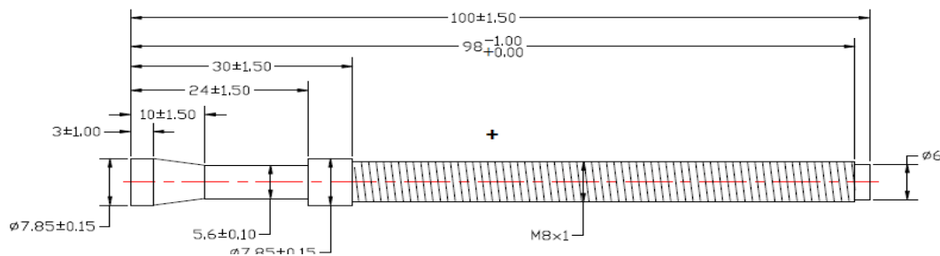
Wedge Anchor Fastener
