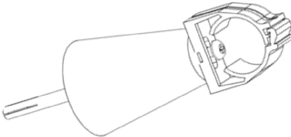
Assembly of PP Clamp 7/8
