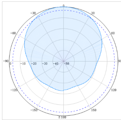
Horizontal (915MHz)
