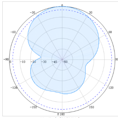
Vertical (915MHz)
