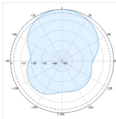
Vertical (866MHz)
