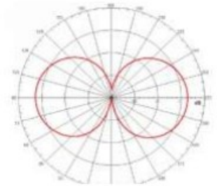
Elevation Pattern Referenced to 0 dBi
